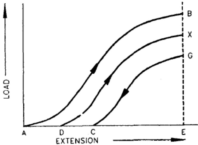
Figure 1: Load Versus Extension Curves
